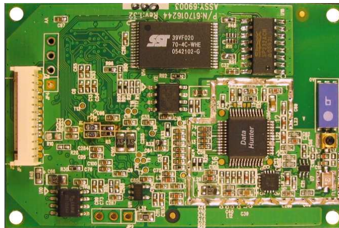
View of Side containing Signal connector and RF connector:
